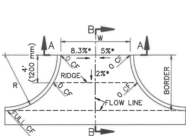
CASE A STANDARD APPROACH
