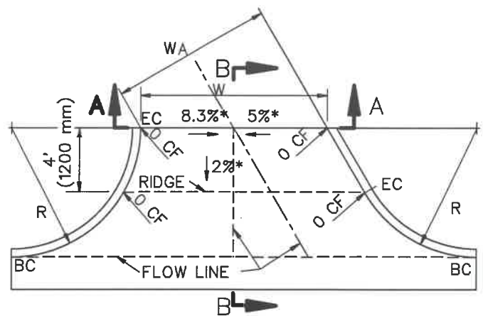
CASE B ANGLED APPROACH
